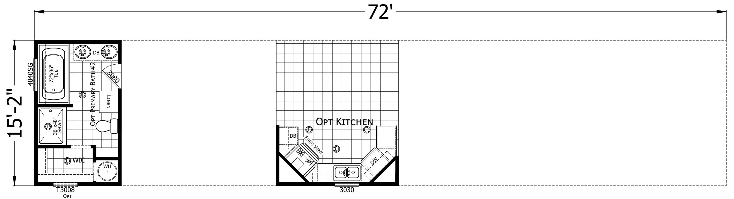
CS1672C-1672H32A6B 3 BEDROOM 2 BATH 72'-0" x 15'-2" 1092 Sq. Ft. TOTAL
