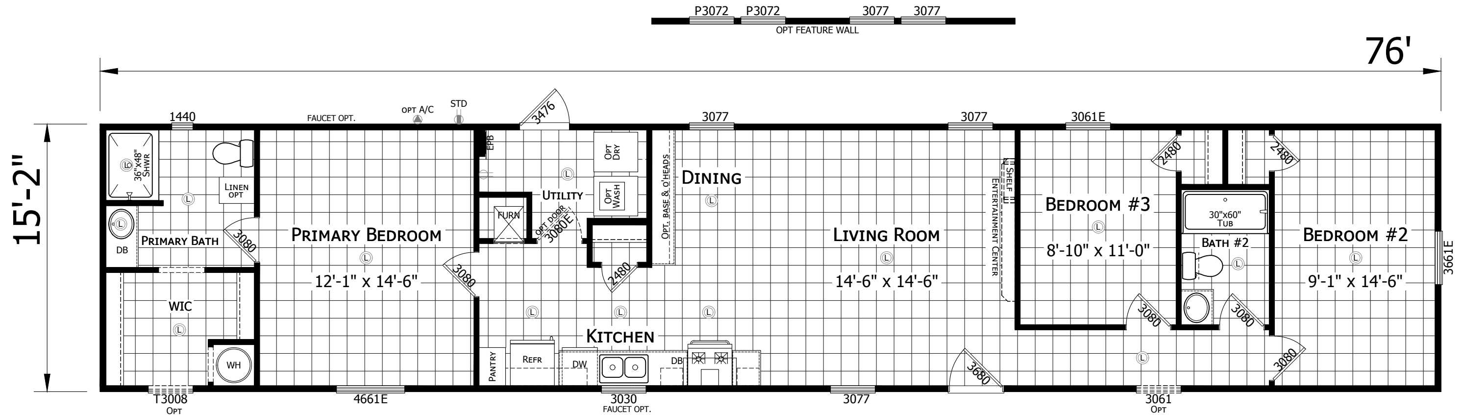
CS1676A-1676H32A6E 3 BEDROOM 2 BATH 76'-0" x 15'-2" 1153 Sq. Ft. TOTAL
