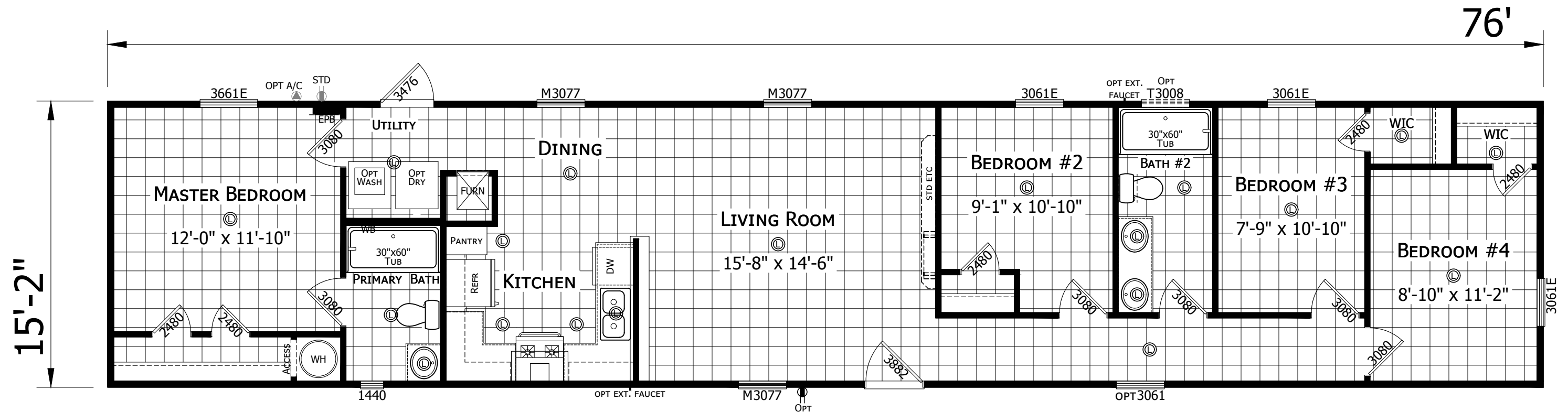
CS1676R-1676H42021 4 BEDROOM 2 BATH 76'-0" x 15'-2" 1153 SQ. FT. TOTAL
