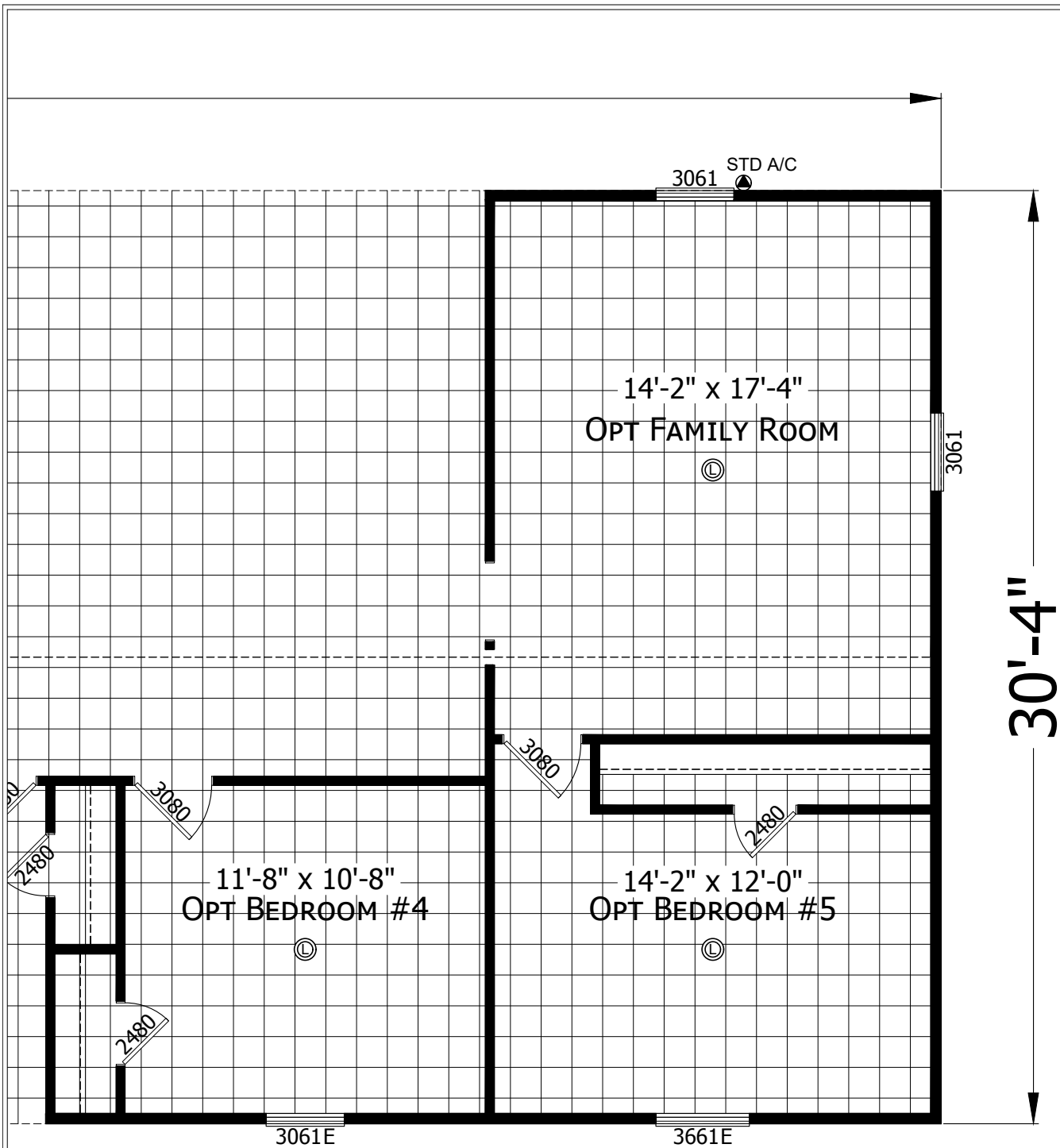
CSD3276L-3276H533273 5 BEDROOM 3 BATH 76'-0" x 30'-4" 2305 Sq. Ft. TOTAL
